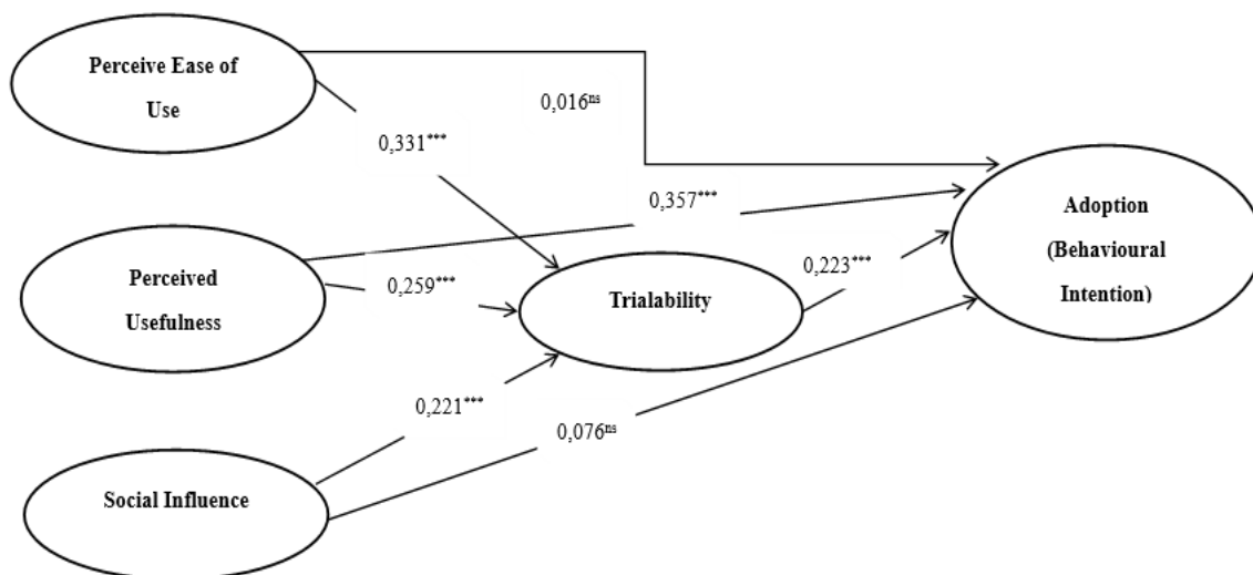
Figure 2. Structural model with path coefficients
